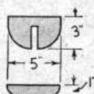
CENTER SECTION LOCK PIECES \frac{3}{8} " PLYWOOD (2 - 3"x5" AND 4 - 1"x5" PIECES NEEDED)
